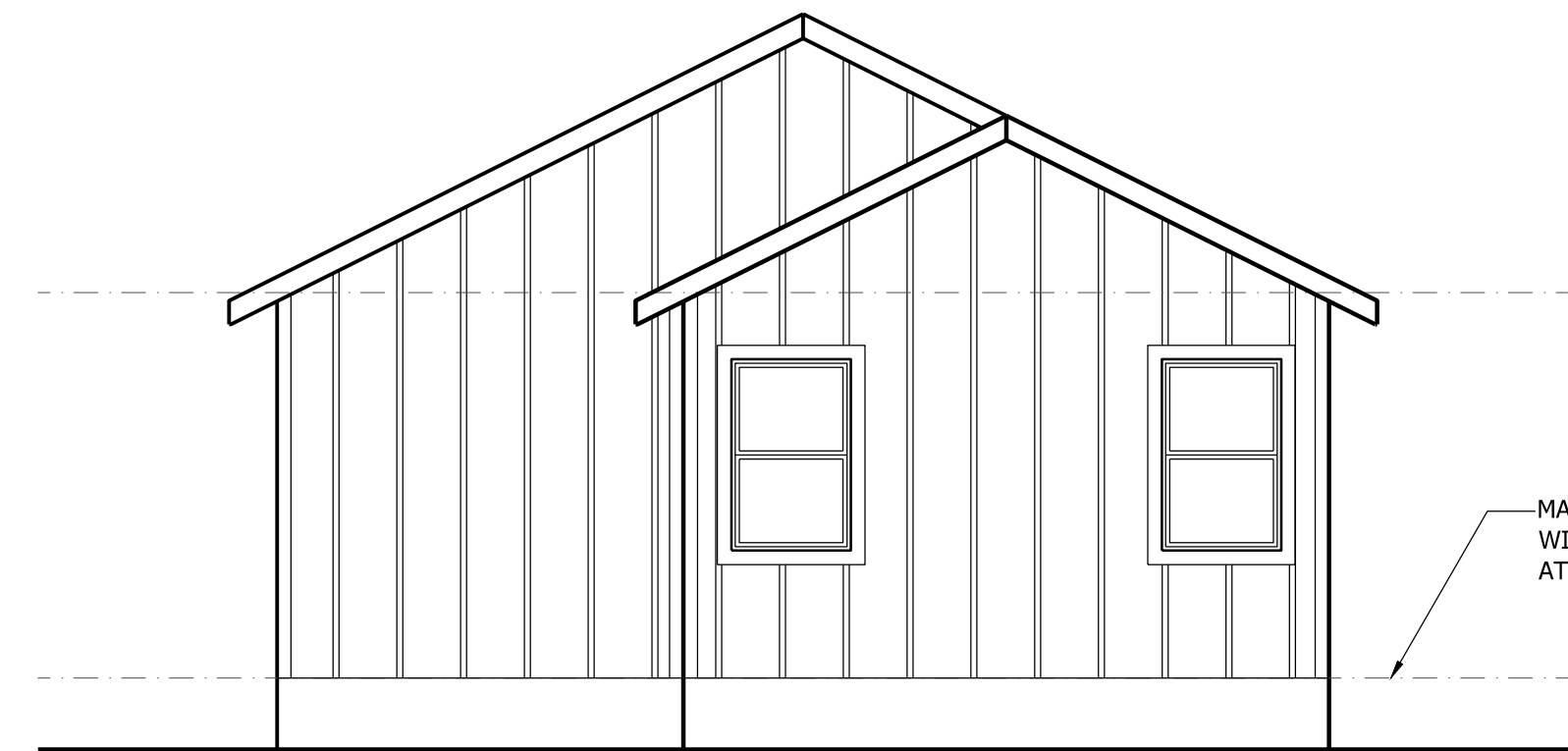
C RIGHT ELEVATION A2.1 1/4" = 1'-0"
