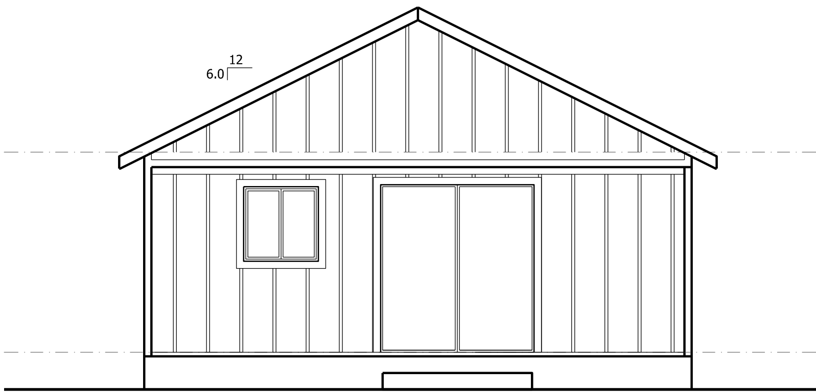
B LEFT ELEVATION A2.1 1/4" = 1'-0"
