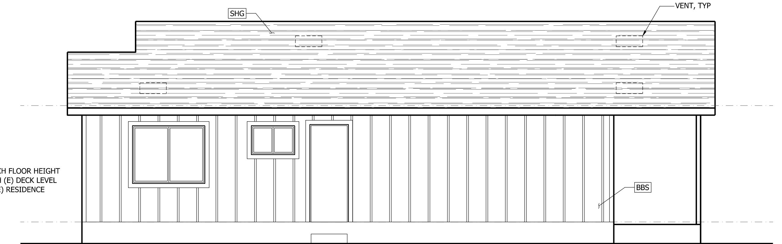
D REAR ELEVATION A2.1 1/4" = 1'-0"
