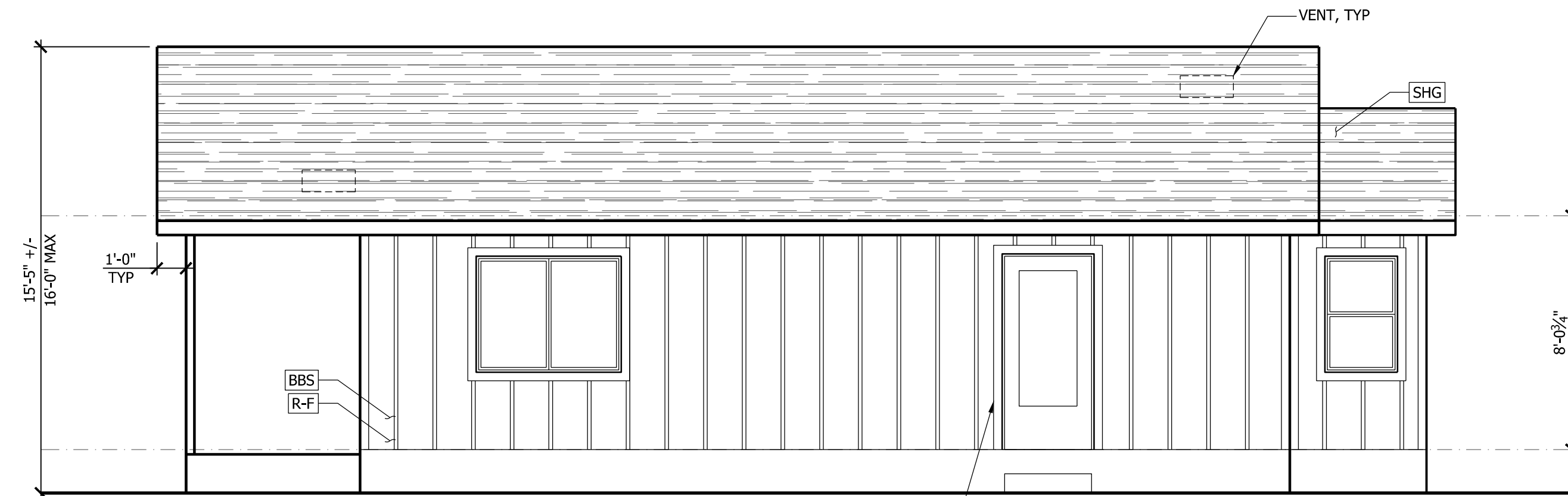
A FRONT ELEVATION A2.1 1/4" = 1'-0"
