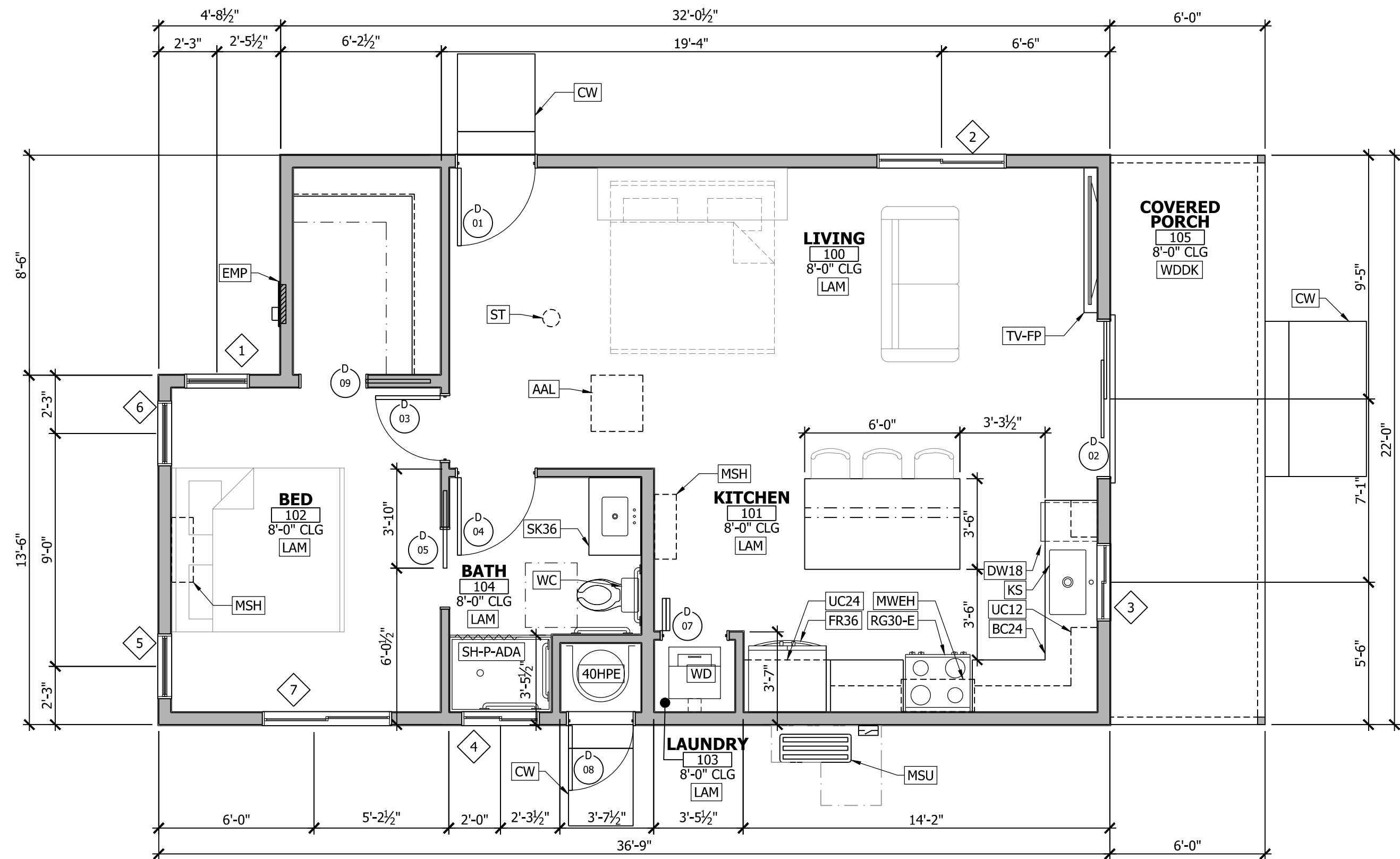
1 FLOOR PLAN A2.1 1/4" = 1'-0"
